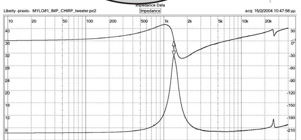
Impedance Response
